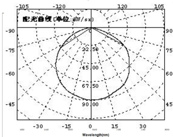
Luminous angle
